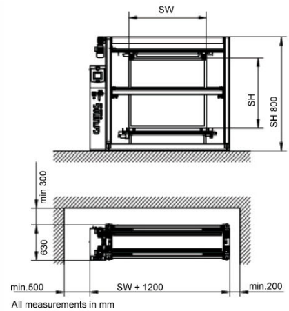
Grünig G-COAT 415 Professional Automatic Coating Machine Schematic
