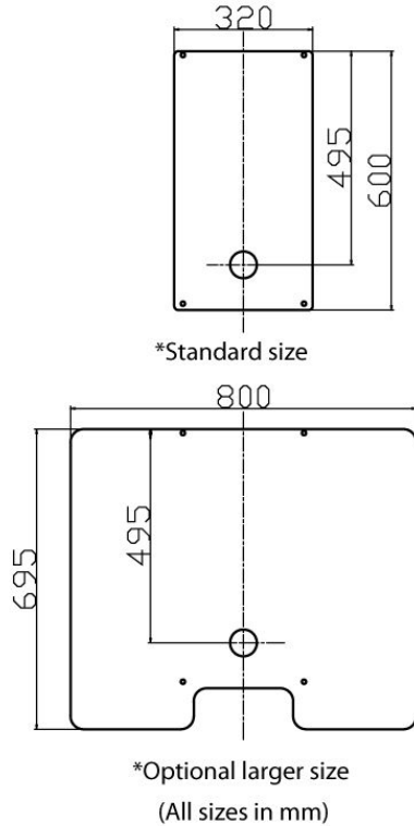
Device Footprint
