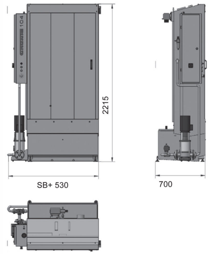
Dimensions (mm)
